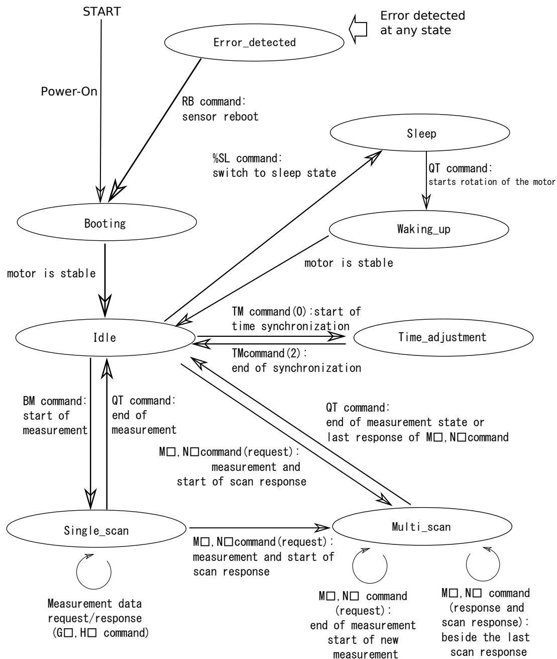
Figure 3.1: Sensor States
