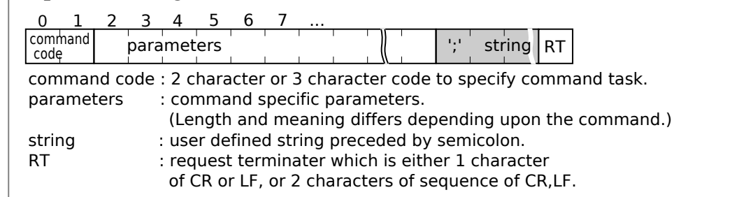
Figure 2.1: Request Message Format
