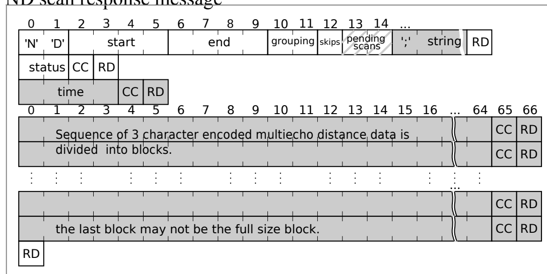
Figure 3.8 : ND Message Format
