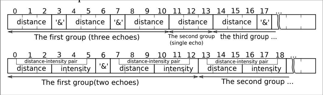
Figure 2.9: Multi- Echo Data Format
