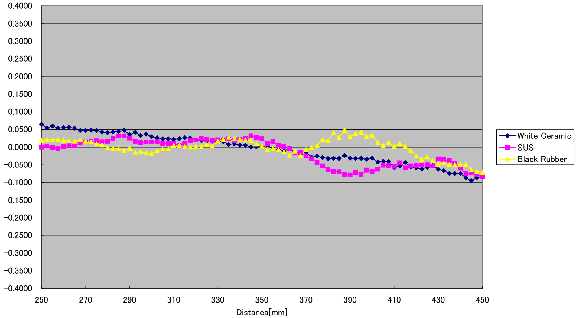
CD5-350-WIDE-800u Linearity(Horizontal 10° )[%FS] (Typical)
