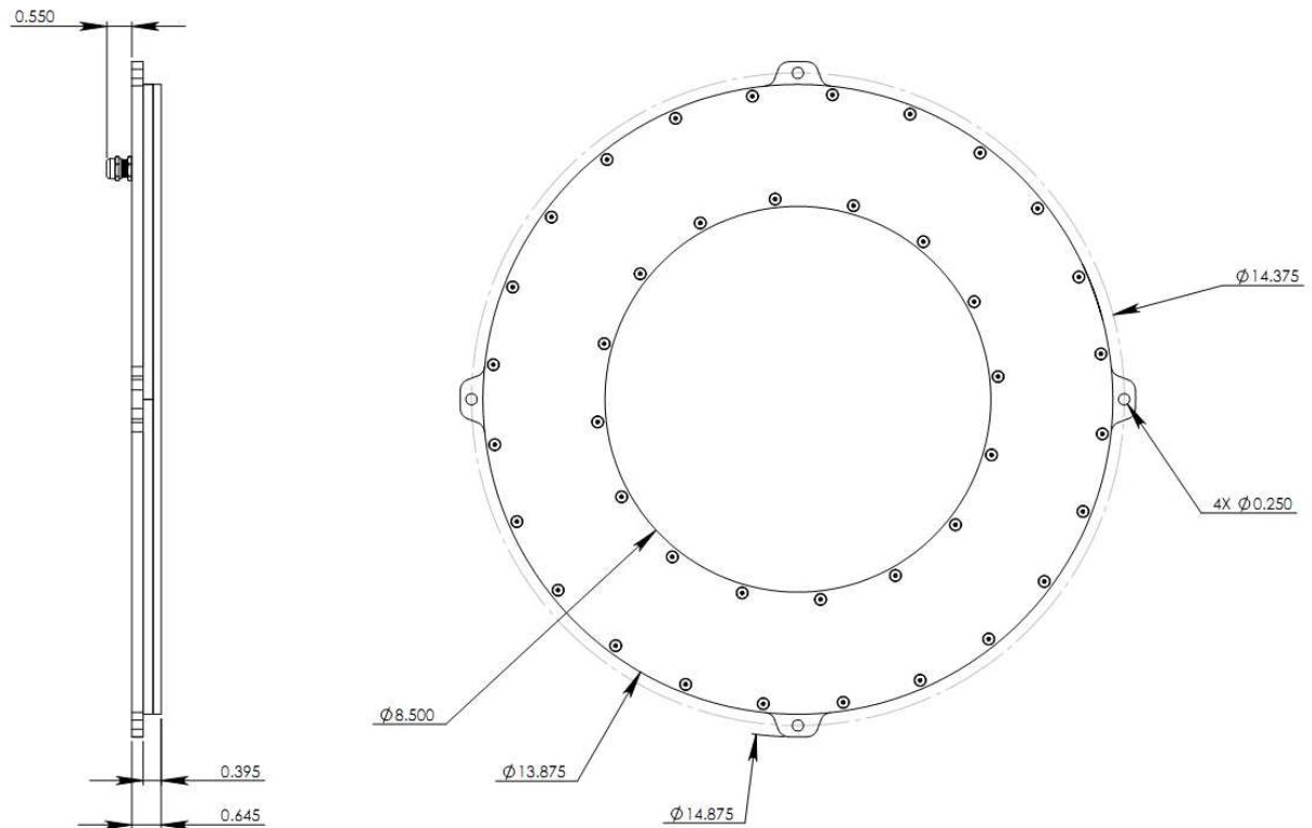
Figure 1: Illustration of illuminator dimensions
