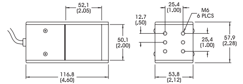
DIMENSIONS ARE IN MILLIMETERS (INCHES)
