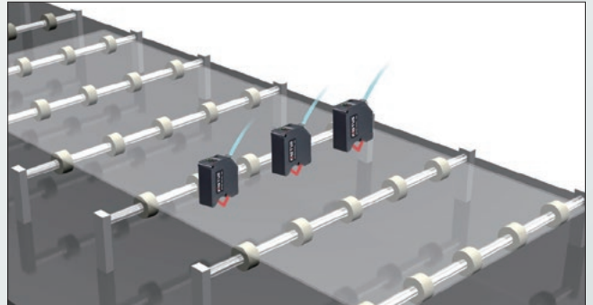
Warping measurement of glass substrates (specular reflection type)
