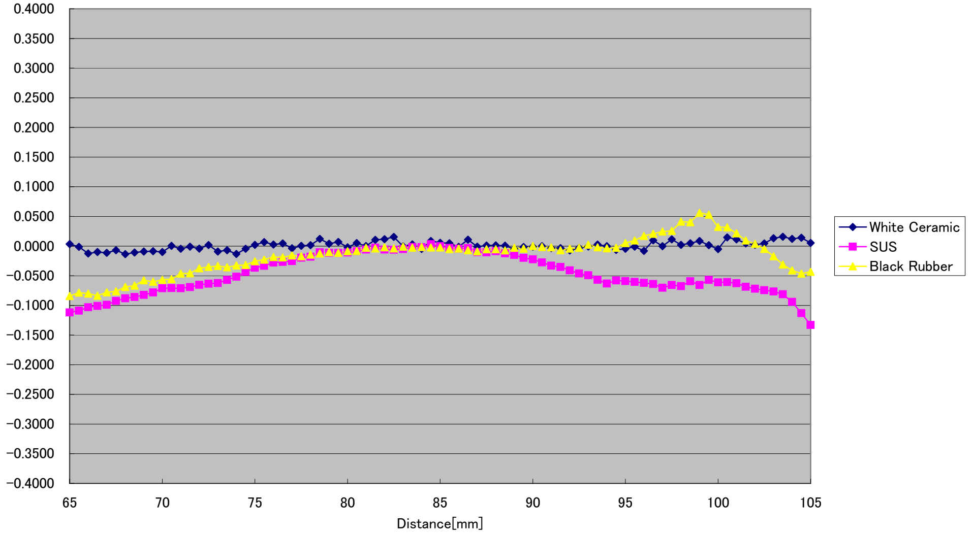
CD5-85-SPOT Linearity( \pm 0^\circ ) [%FS] (Typical)
