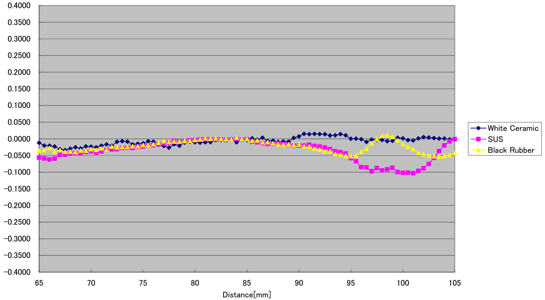
CD5-85-SPOT Linearity(Vertical -10° )[%FS] (Typical)
