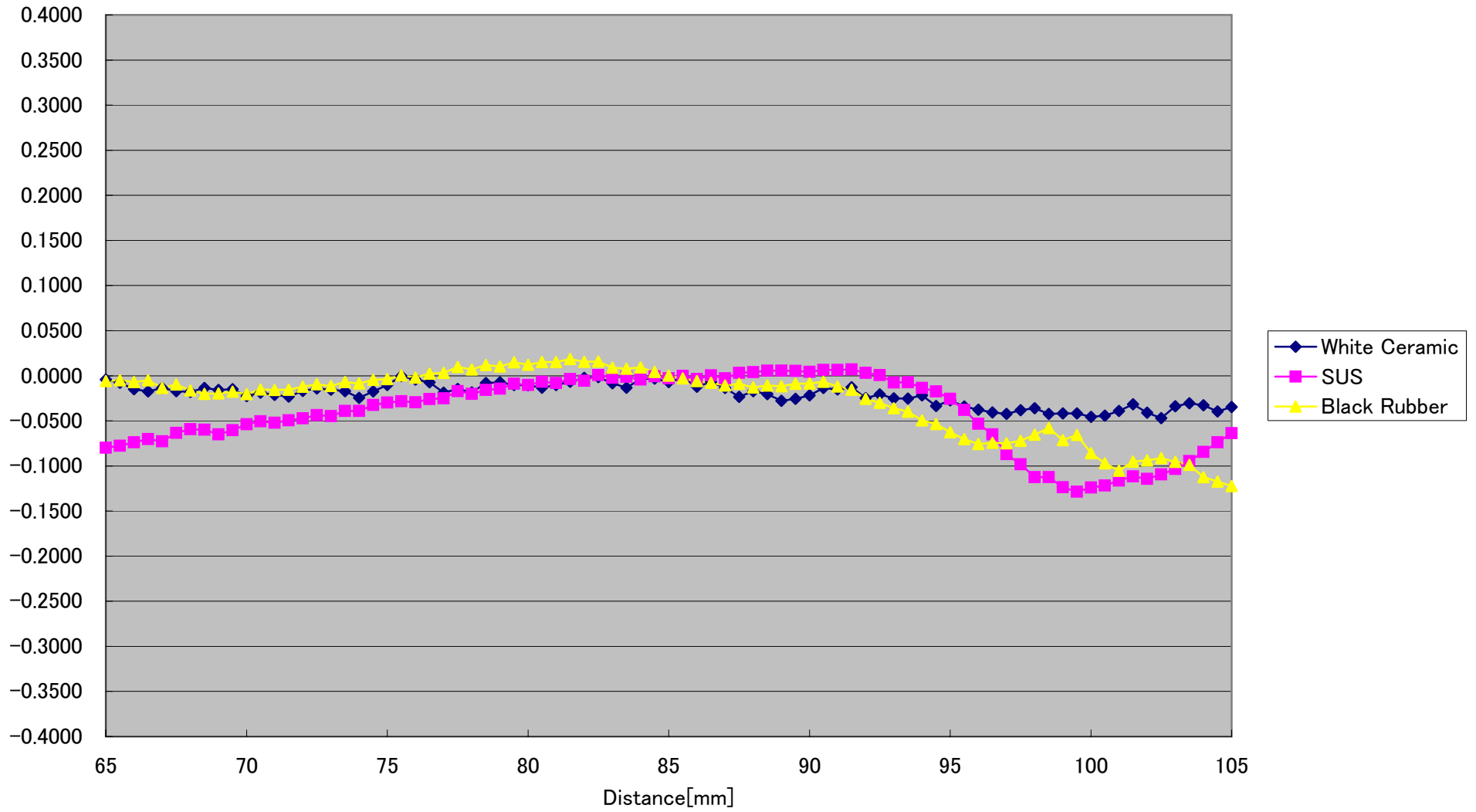
CD5-85-SPOT Linearity(Horizontal 10° )[%FS] (Typical)
