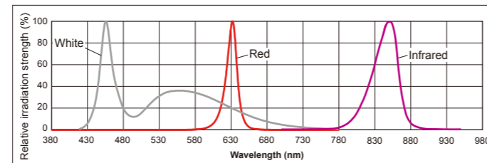
■ Specular Distribution Diagram
