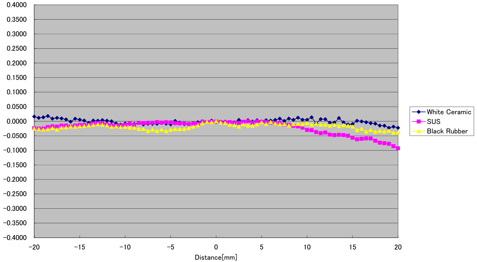
CD5-85-WIDE Linearity(Horizontal 10° )[%FS] (Typical)
