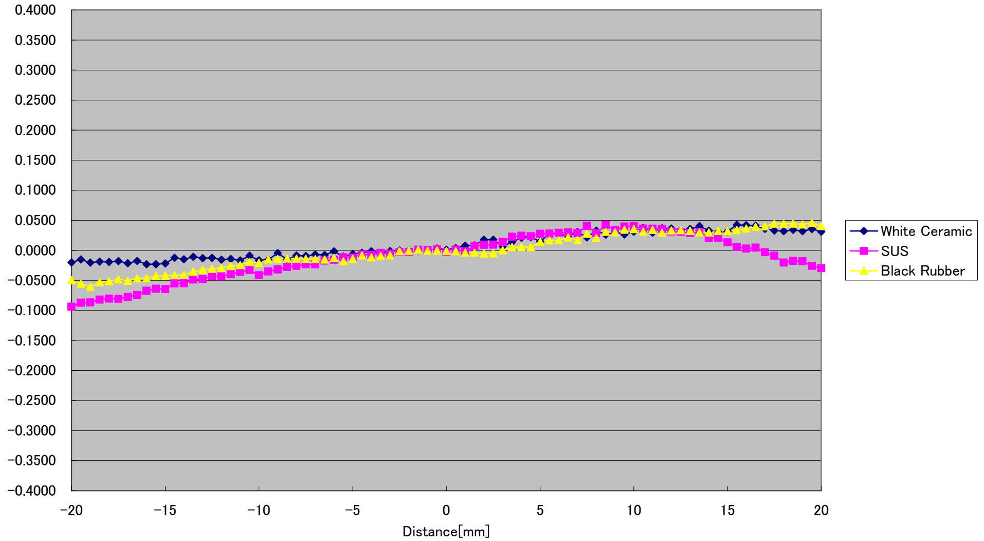
CD5-85-WIDE Linearity(Vertical -10^\circ )[%FS] (Typical)
