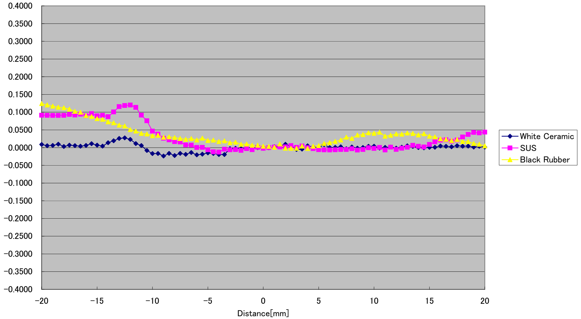
CD5-85-WIDE Linearity(Vertical +10° )[%FS] (Typical)
