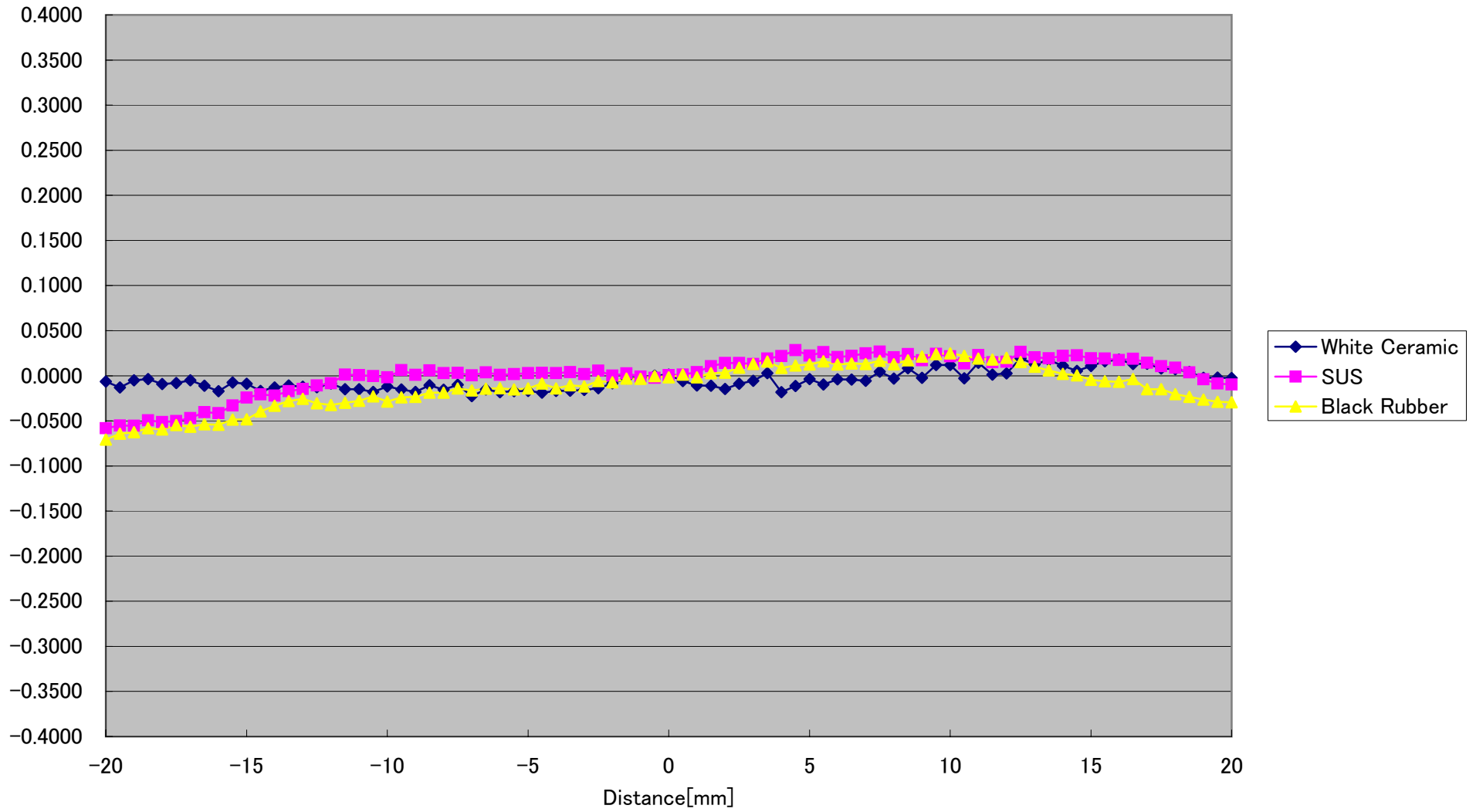
CD5-85-WIDE Linearity( \pm 0^\circ ) [%FS] (Typical)
