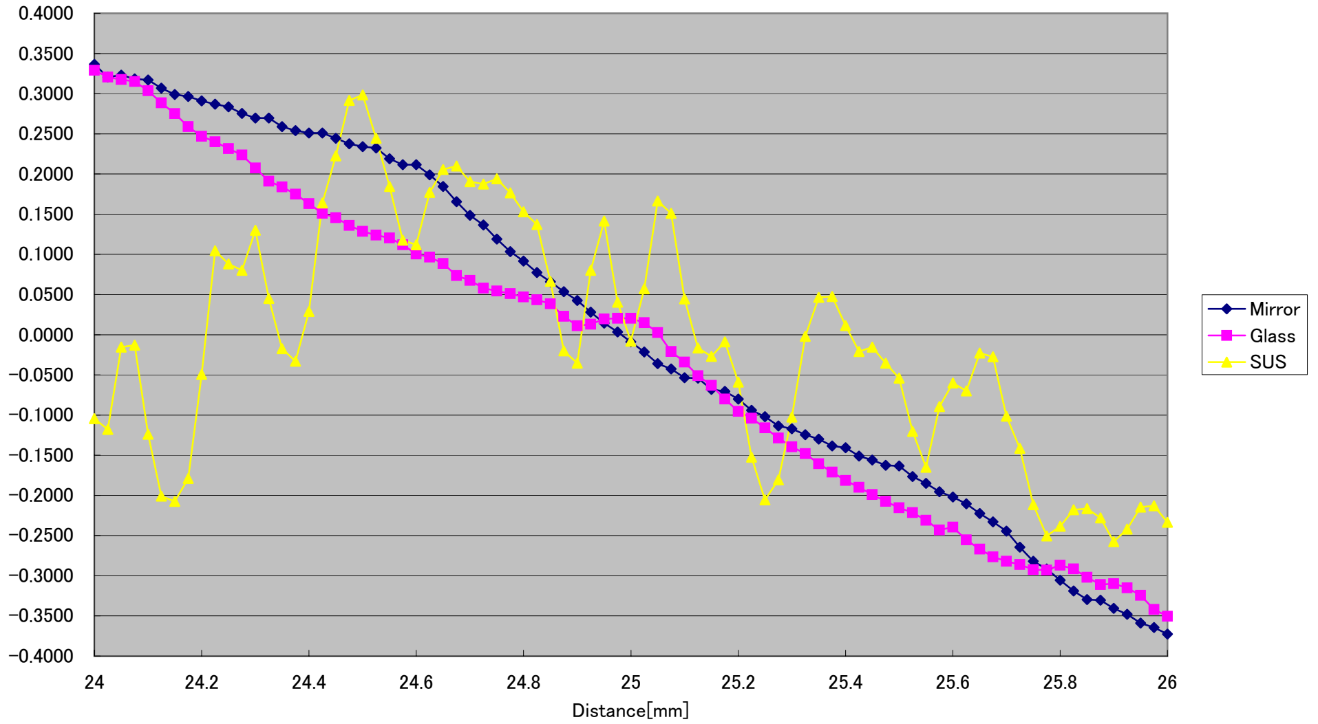
CD5-25-SPOT Linearity(Vertical -0.2^\circ )[[%FS] (Typical)
