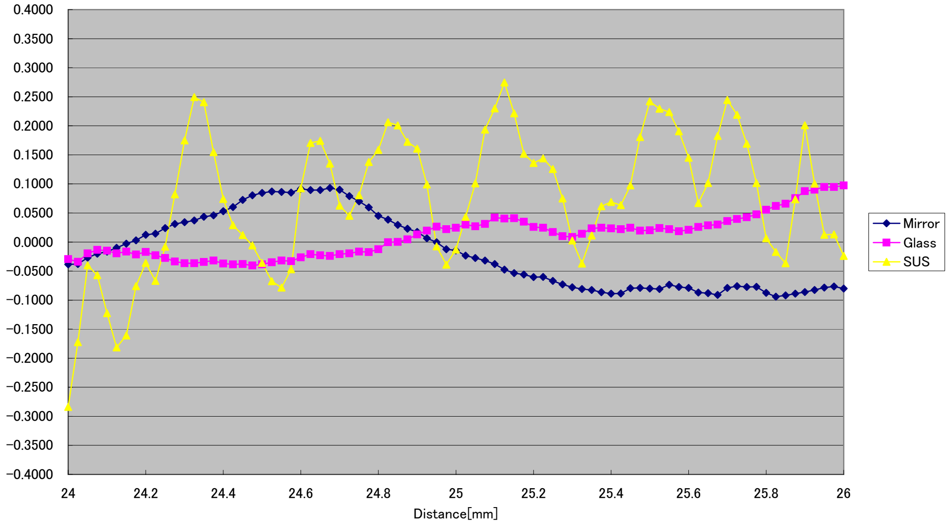
CD5-25-SPOT Linearity(Horizontal 0.2° )[%FS] (Typical)
