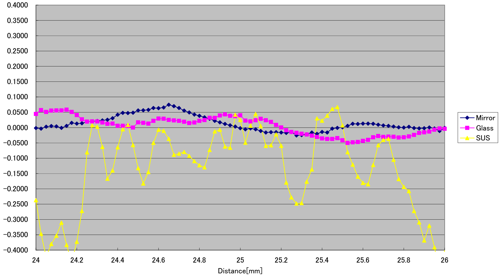
CD5-25-SPOT Linearity( \pm 0^\circ )[%FS] (Typical)
