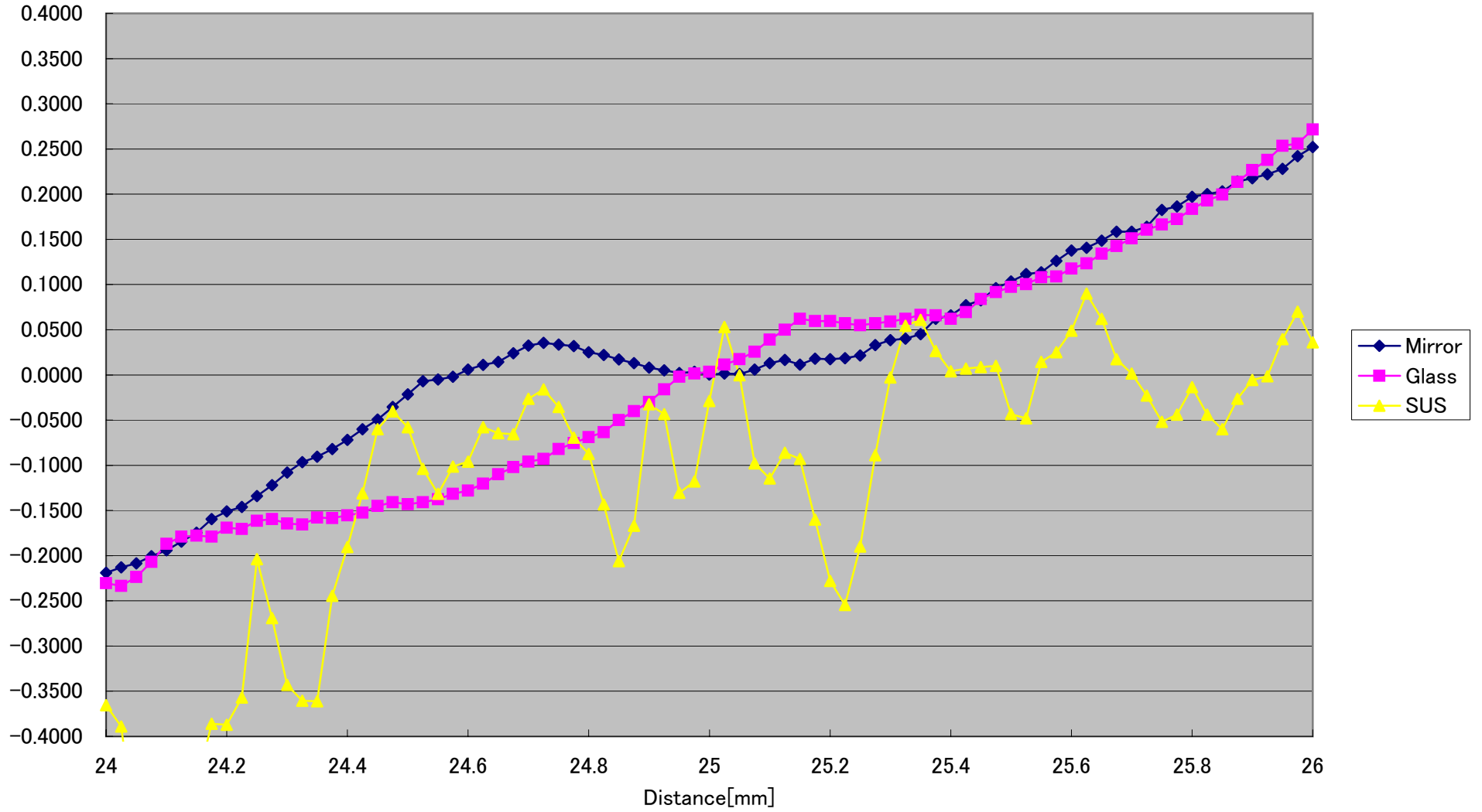
CD5-25-SPOT Linearity(Vertical +0.2° )[%FS] (Typical)
