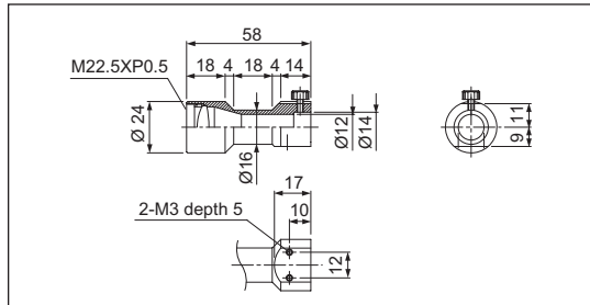
Dimensions of HL-24-21 (Unit: mm)
