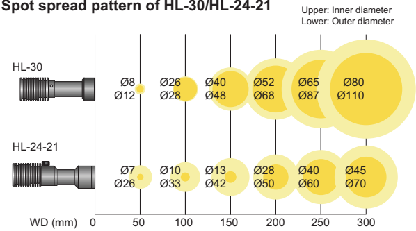
Spot spread pattern of HL-30/HL-24-21
