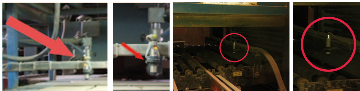
Pics.1 - 4: Example of installations of M.D.'s photoelectric sensors in kilns.
