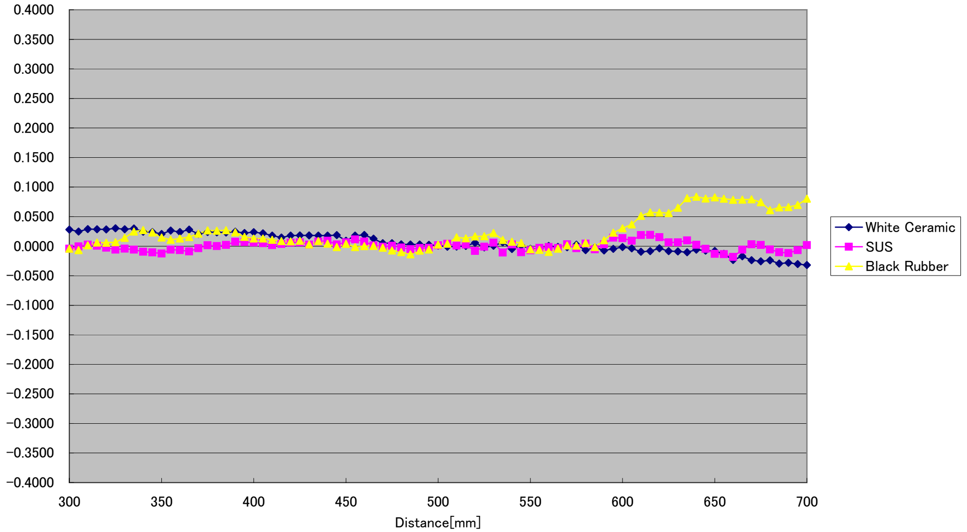
CD5-500-WIDE Linearity(Vertical -10^\circ )[%FS] (Typical)
