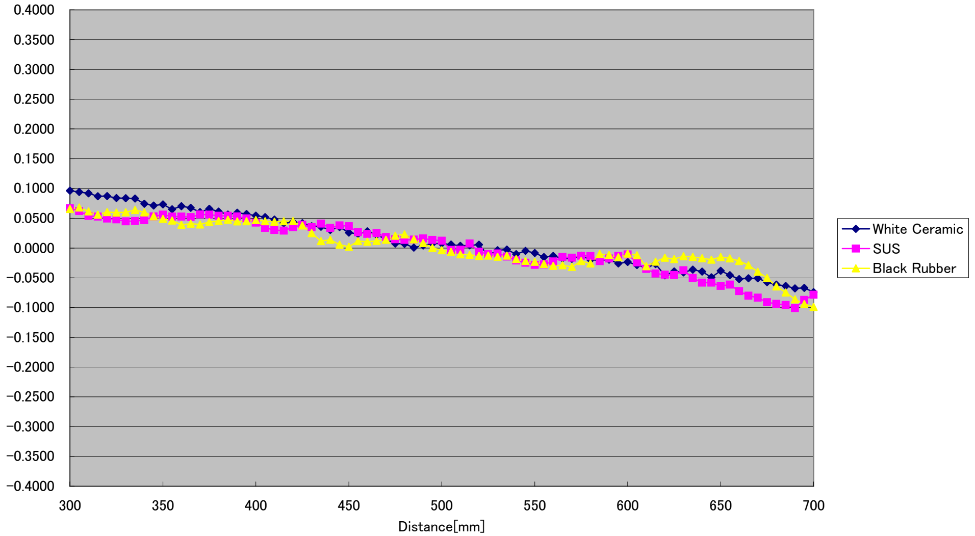
CD5-500-WIDE Linearity(Horizontal 10° )[%FS] (Typical)
