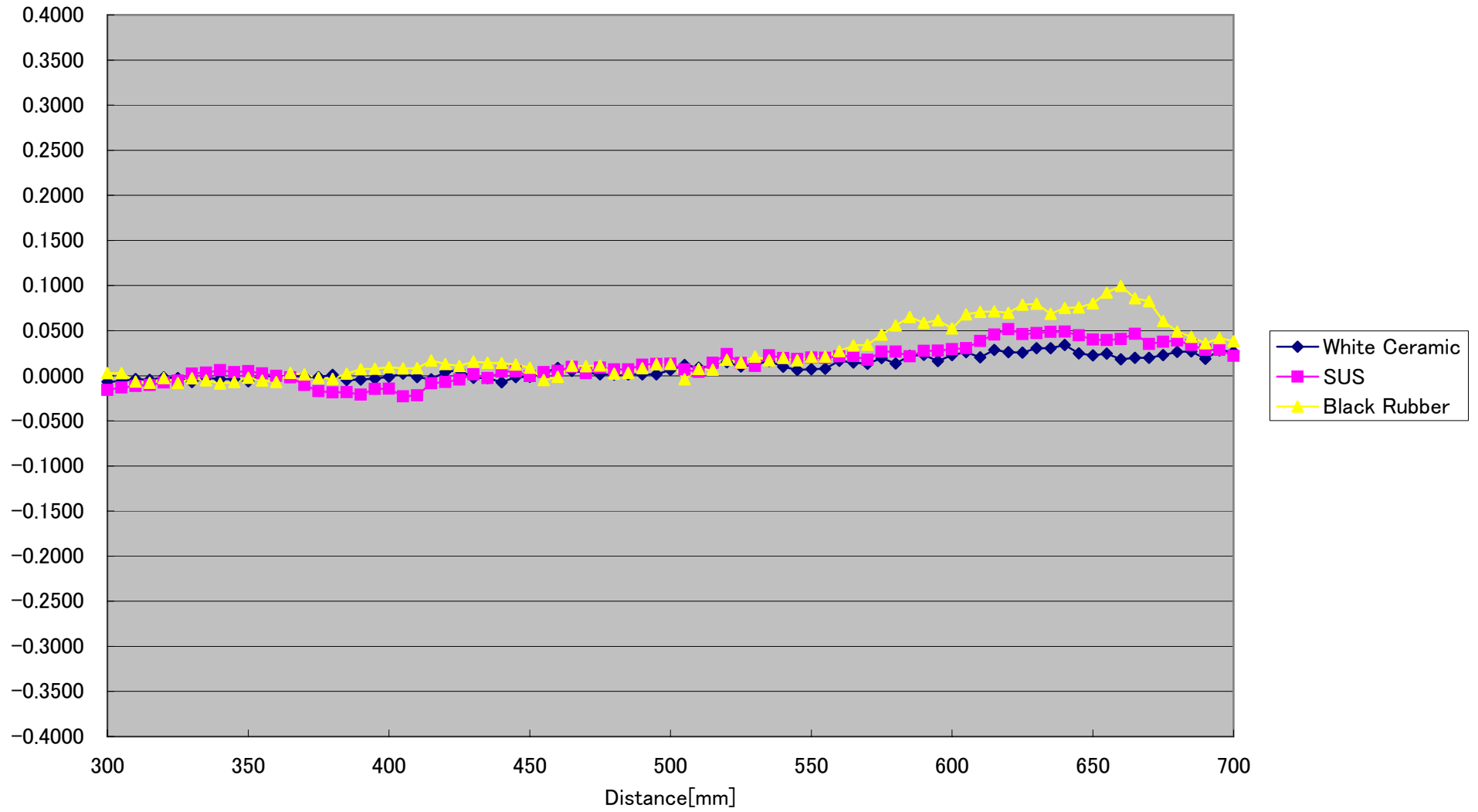
CD5-500-WIDE Linearity(Vertical +10° )[%FS] (Typical)
