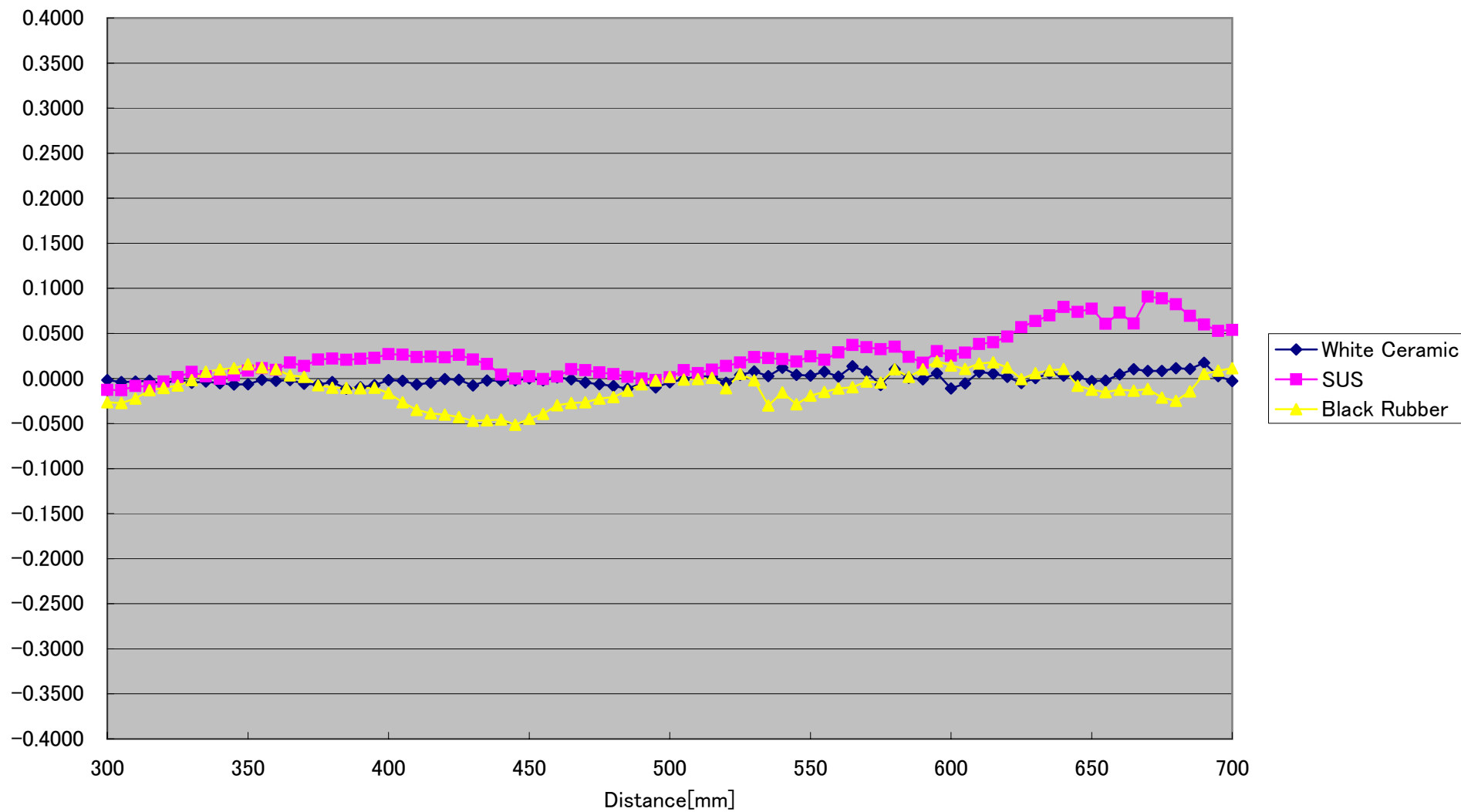
CD5-500-WIDE Linearity( \pm 0^\circ )[%FS] (Typical)
