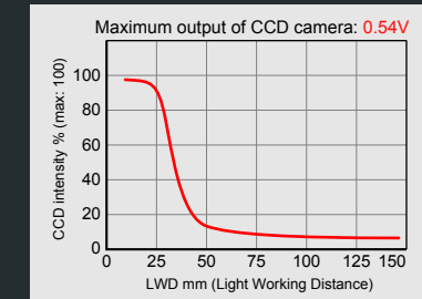
CCD intensity vs LWD
