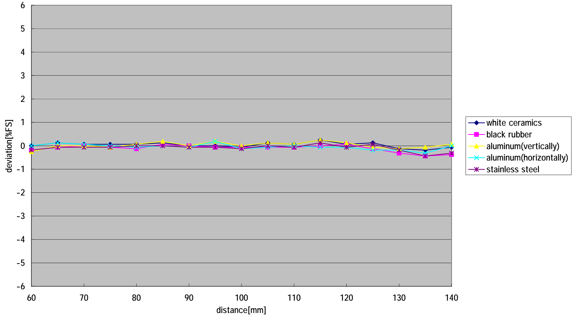
CD3-100 (typical)
