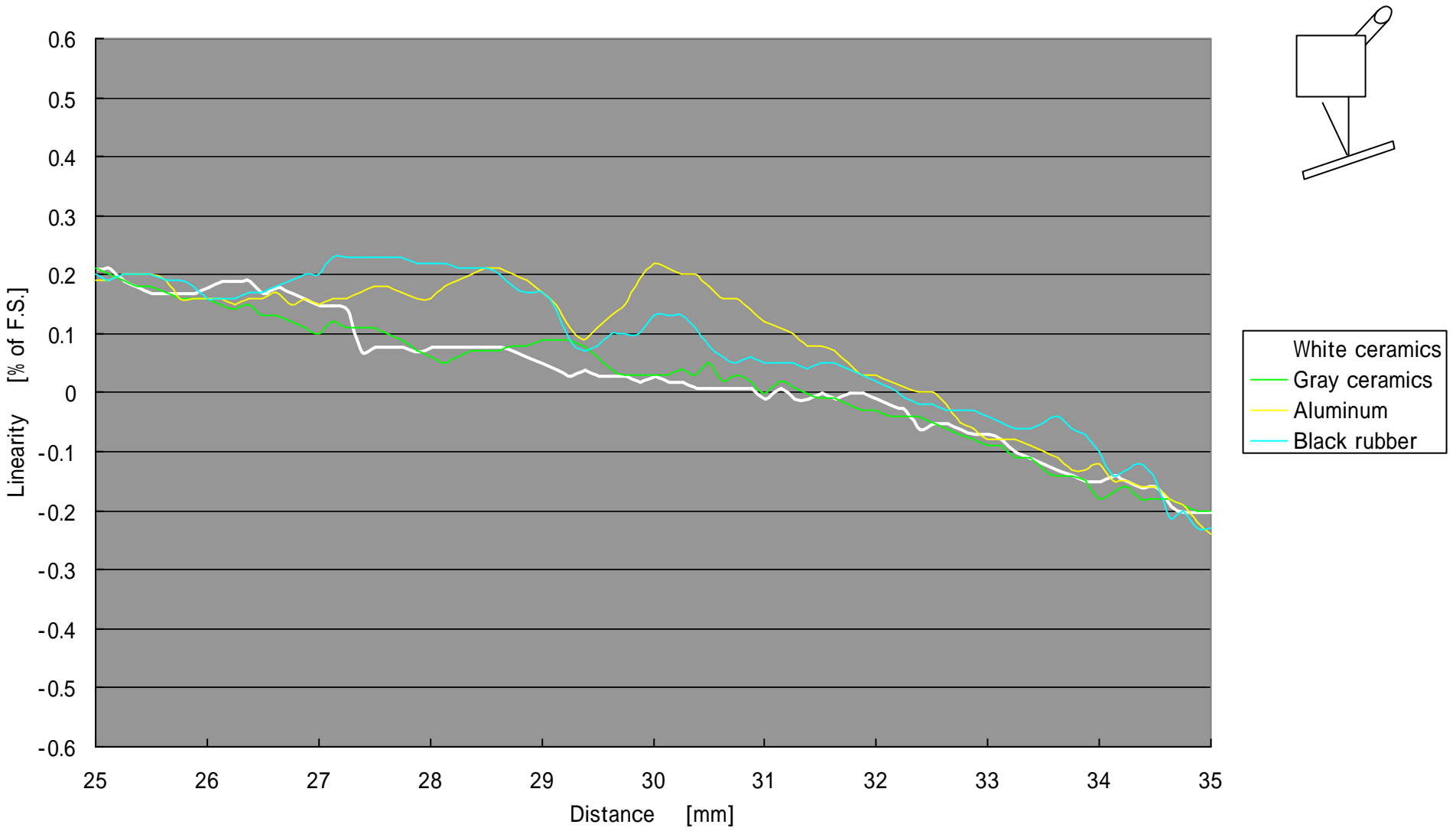
CD4-30 [+10 °] (Typical)
