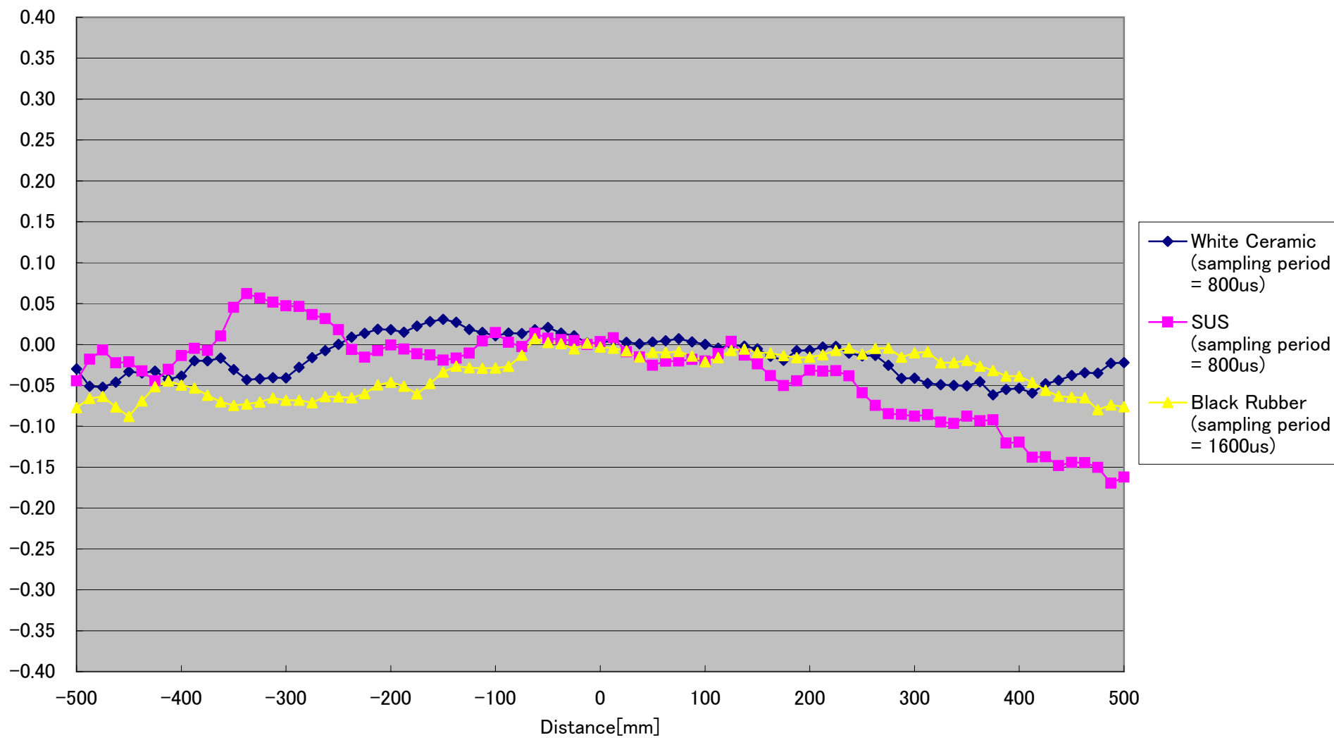
CD5-W2000 Linearity ( \pm 0^\circ ) [%FS]
