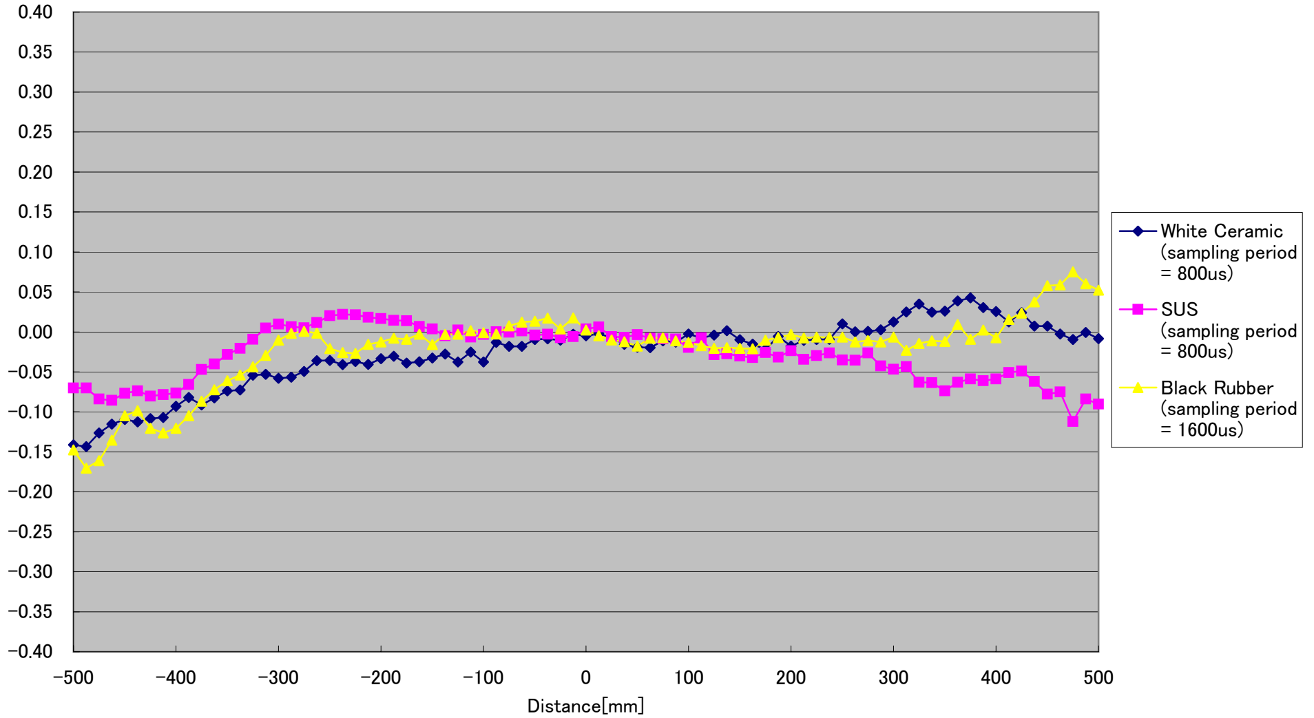
CD5-W2000 Linearity (Vertical -10^\circ ) [%FS]
