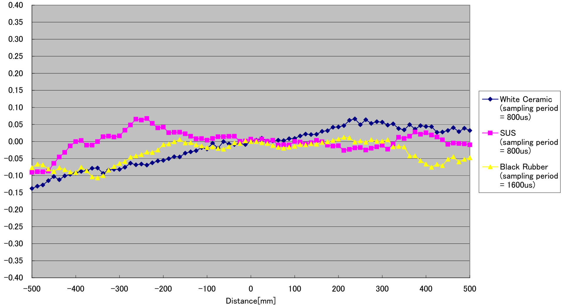
CD5-W2000 Linearity (Horizontal 10° )[%FS]
