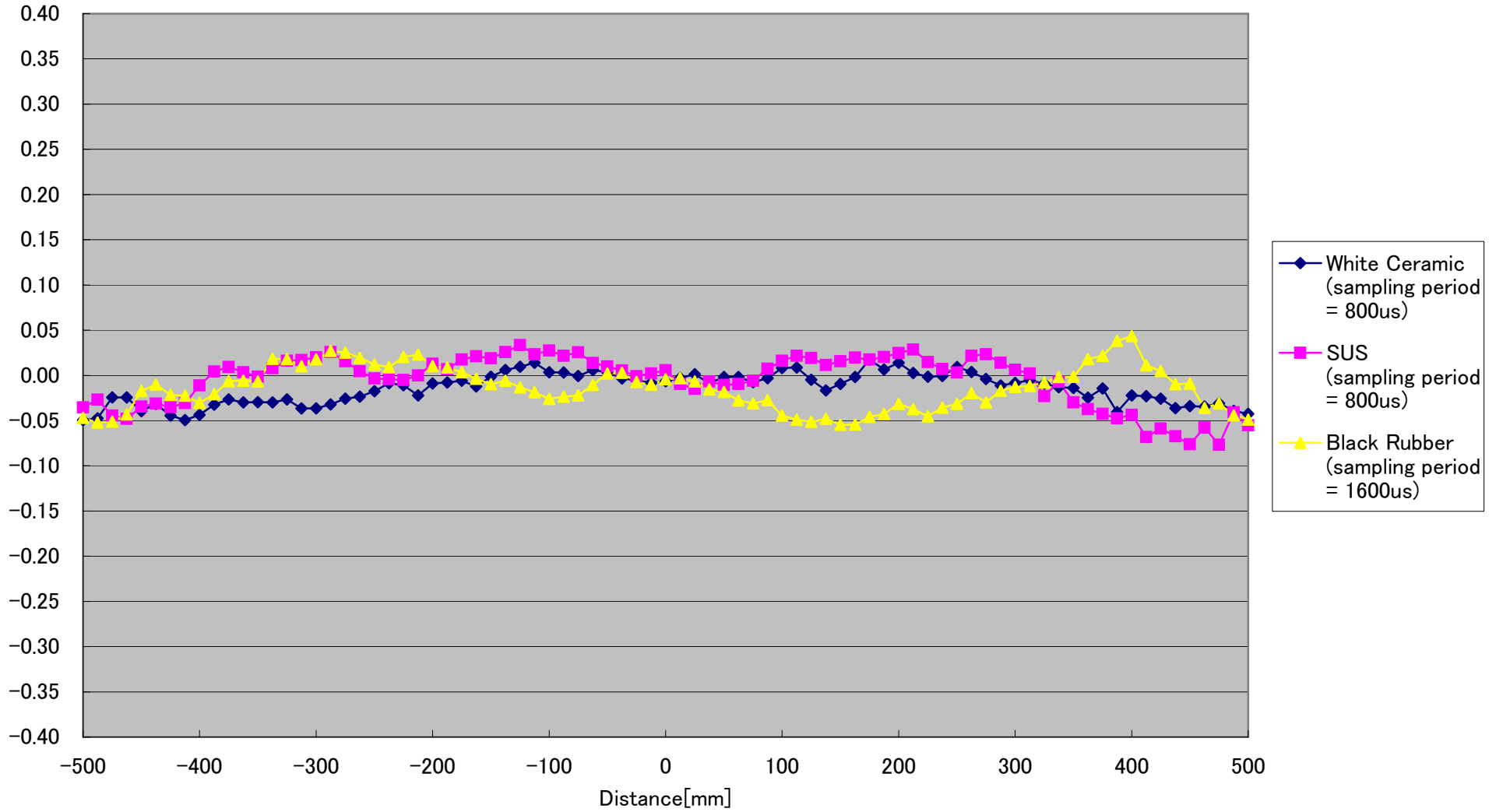
CD5-W2000 Linearity (Vertical +10° )[%FS]
