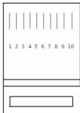
Pin Out for RJ45 Plug
