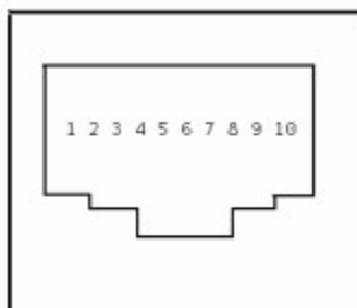
Pin Out for RJ45 Jack
