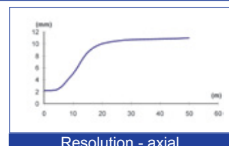
Resolution - axial
