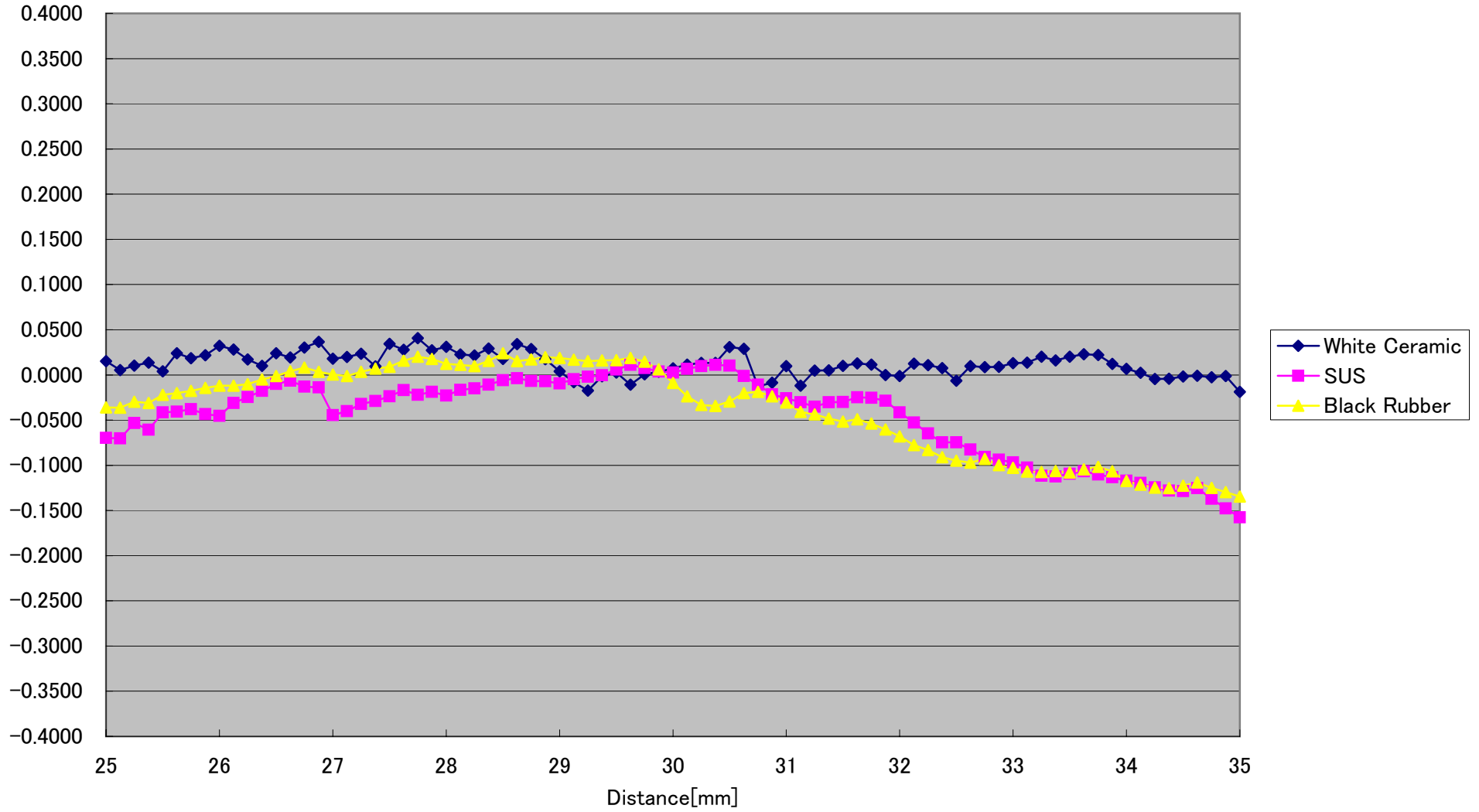
CD5-30-SPOT Linearity(Vertical -10° )[%FS] (Typical)
