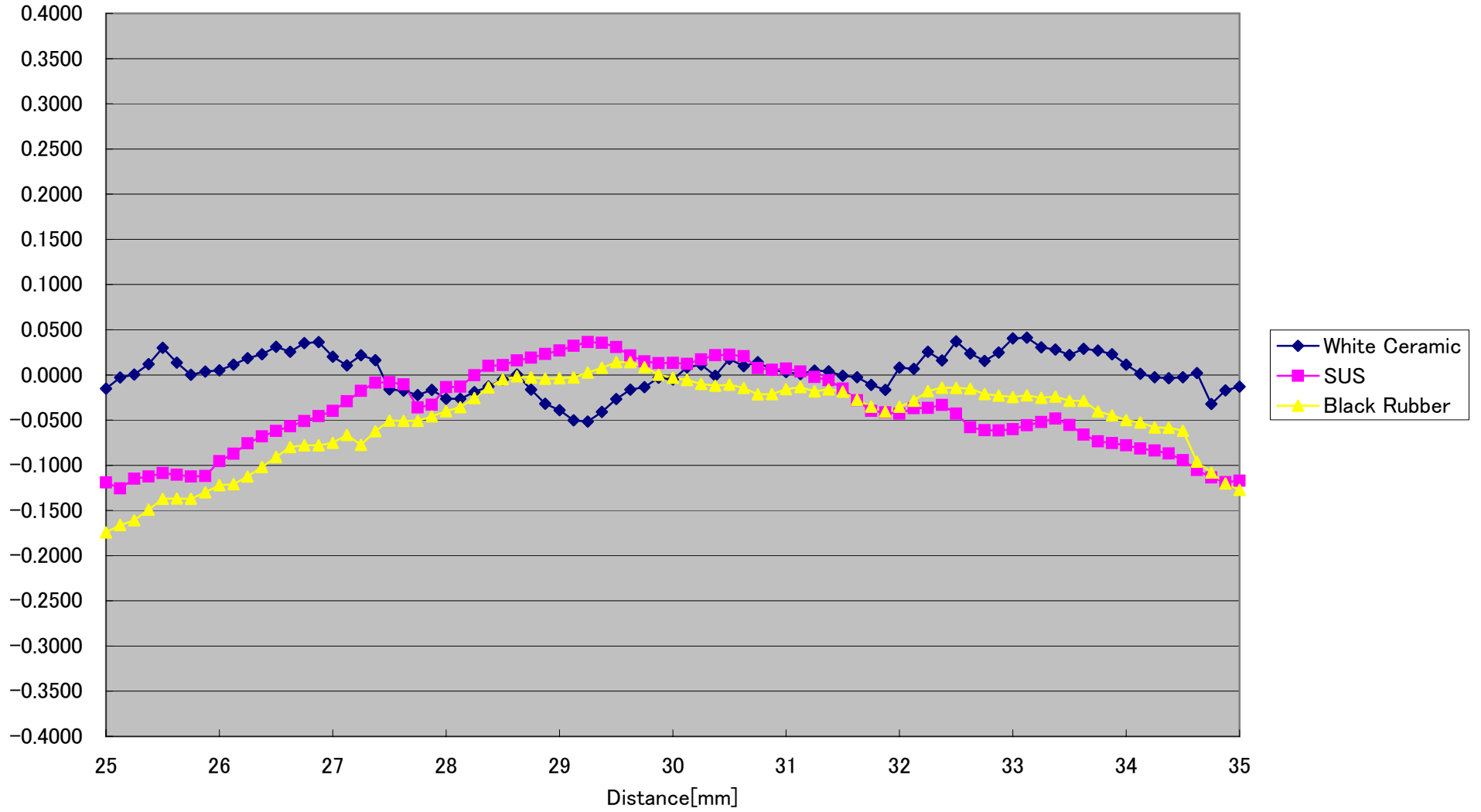
CD5-30-SPOT Linearity(Horizontal 10° )[%FS] (Typical)
