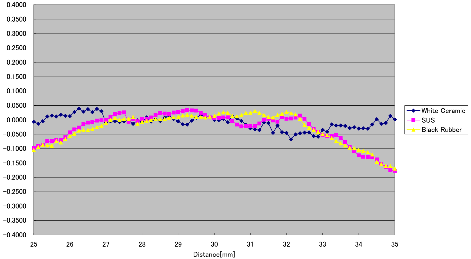
CD5-30-SPOT Linearity( \pm 0^\circ ) [%FS] (Typical)
