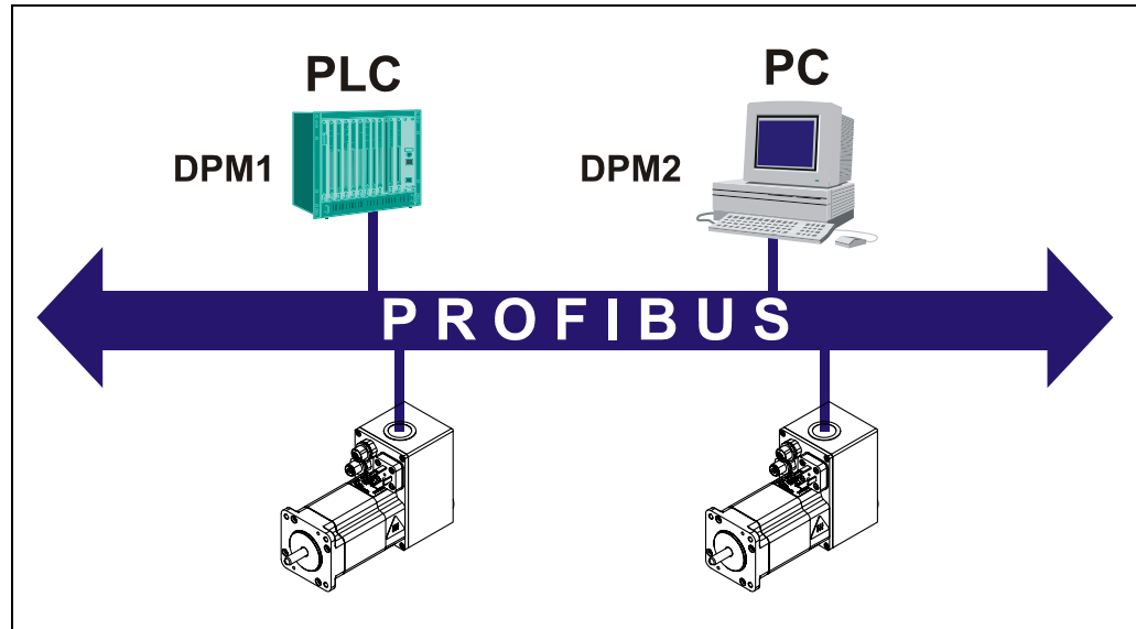
Figure 1: Drives on the field bus
